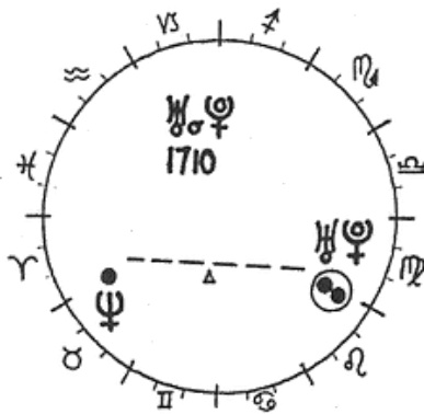
Uranus conjunct Pluto 1710
