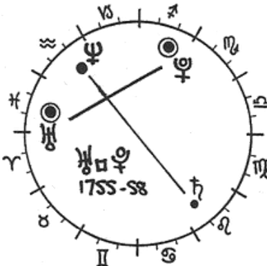
Uranus square Pluto 1755-58
