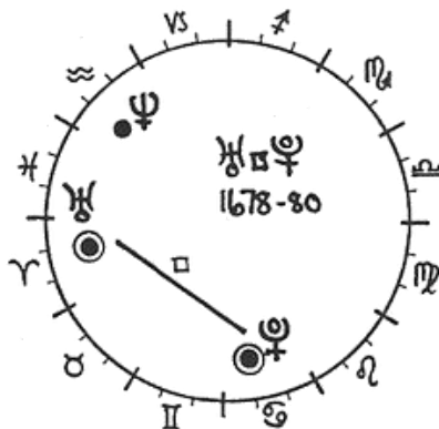
Uranus square Pluto 1678-80
